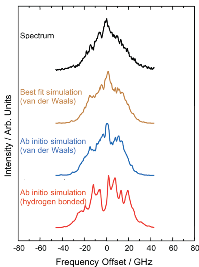
FIG. 19 Rotational contours for the phenol...argon S_1 \leftarrow S_0 transition: (a) for the van der Waals above-ring structure, (b) for the hydrogen-bonded local minimum structure. Reproduced from ref. 231 (improved fitting compared to ref. 232 )
