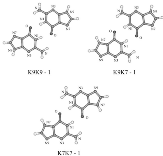
FIG. 17 Structures of the guanine dimer. Reproduced from ref. 185 with permission
